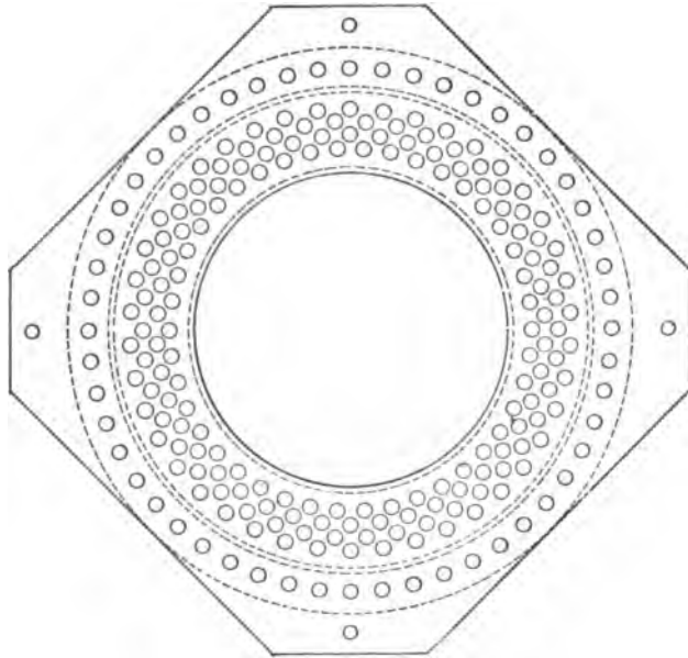
FIG. 166.—Plan View of the Upper Plate of the Lever of Water Chamber of the Thornycroft Boiler. Comparison of this with previous cut gives an idea of the spread of the tubes.
